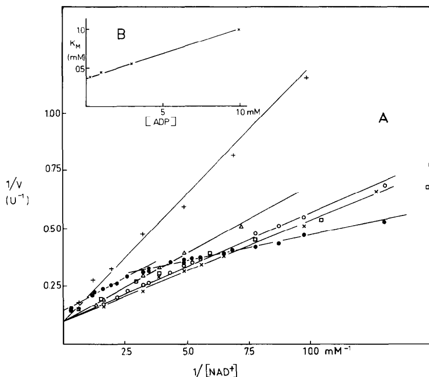
Fig. 2. A: Lineweaver-Burk plot for the reaction with NAD^+ . Initial rate ( v ) measurements given in international units ( U = \mu\text{moles}/\text{mg}\cdot\text{min} ) in 0.067 M phosphate buffer, pH 7.6, at 8.5 mM glutamate and with ADP concentrations of 10 ( +\text{---}+ ), 3 ( \Delta\text{---}\Delta ), 1 ( \square\text{---}\square ), 0.3 ( \times\text{---}\times ) and 0.025 mM ( \bullet\text{---}\bullet ) is the control in the absence of ADP. B (Insert): Secondary plot of K_m (from A) against ADP concentration.
